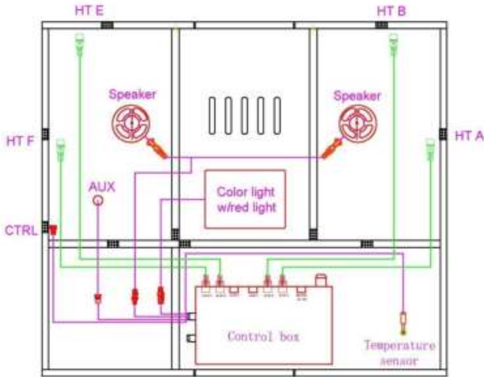
Roof Panel
