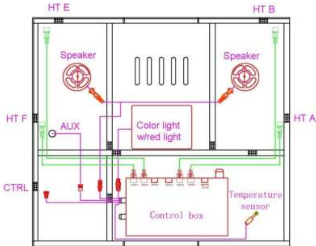
Roof Panel
